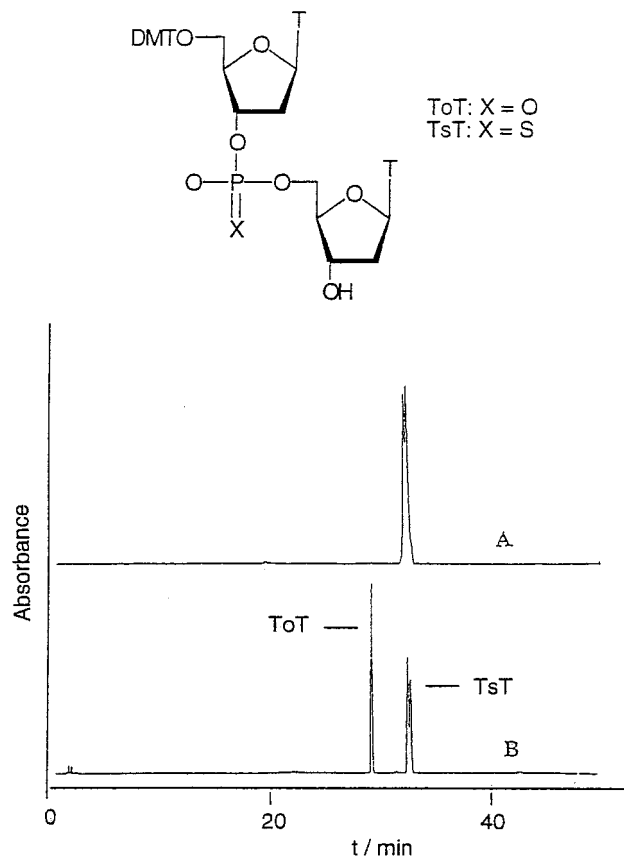
Figure 1. The reverse-phase HPLC analyses of dinucleotide phosphorothioate (TsT) and phosphodiester (ToT). (A) Sulfurization was carried out using 4 equiv of ADTT for 1 min; (B) co-injection of the dinucleotide phosphodiester (ToT) and phosphorothioate (TsT).
