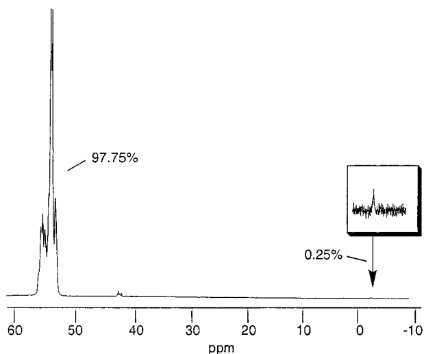
Figure 2. Analysis of the crude 18mer oligonucleotide phosphorothioate (GEM-231) by ^{31}\text{P} NMR.
