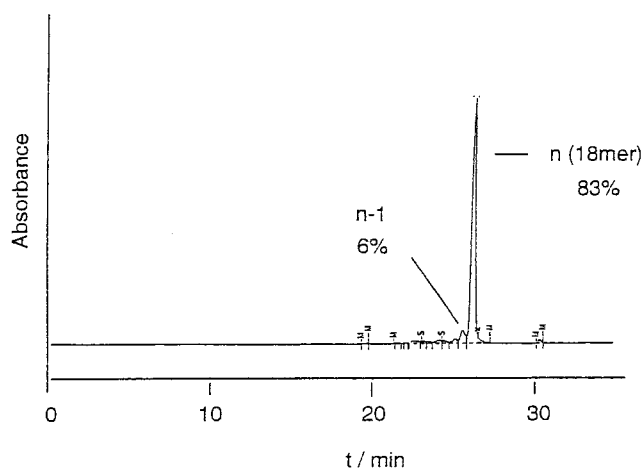
Figure 3. Analysis of the crude 18mer oligonucleotide phosphorothioate (GEM-231) by capillary gel electrophoresis.
